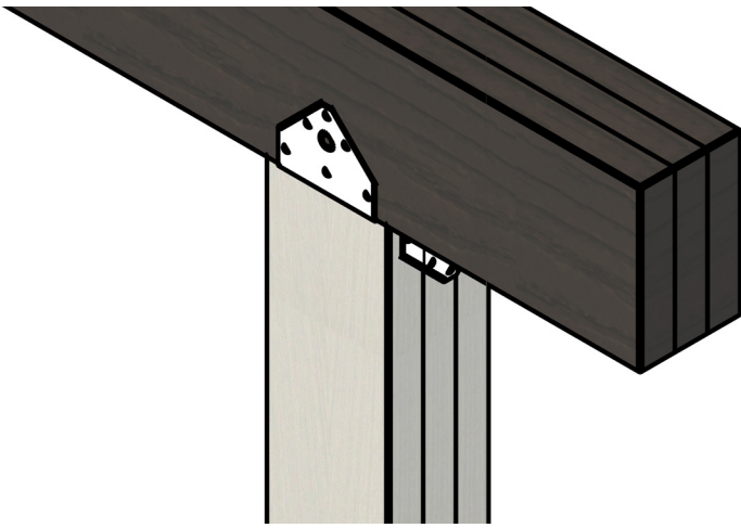
FIGURE 6: 3-Ply beam with post cap attachment
