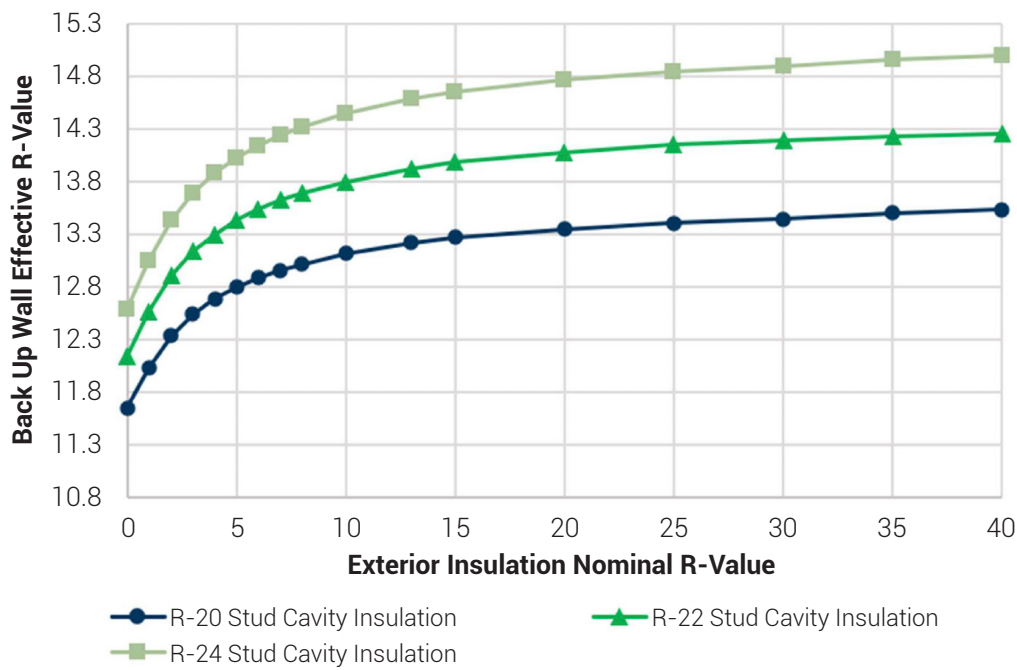
Figure A1: Effective R-Values of Interior Insulated Steel-Frame Back-Up Wall Assemblies with R-20, R-22 and R-24 Insulation in the Stud Cavity and Various Exterior Insulation Levels
