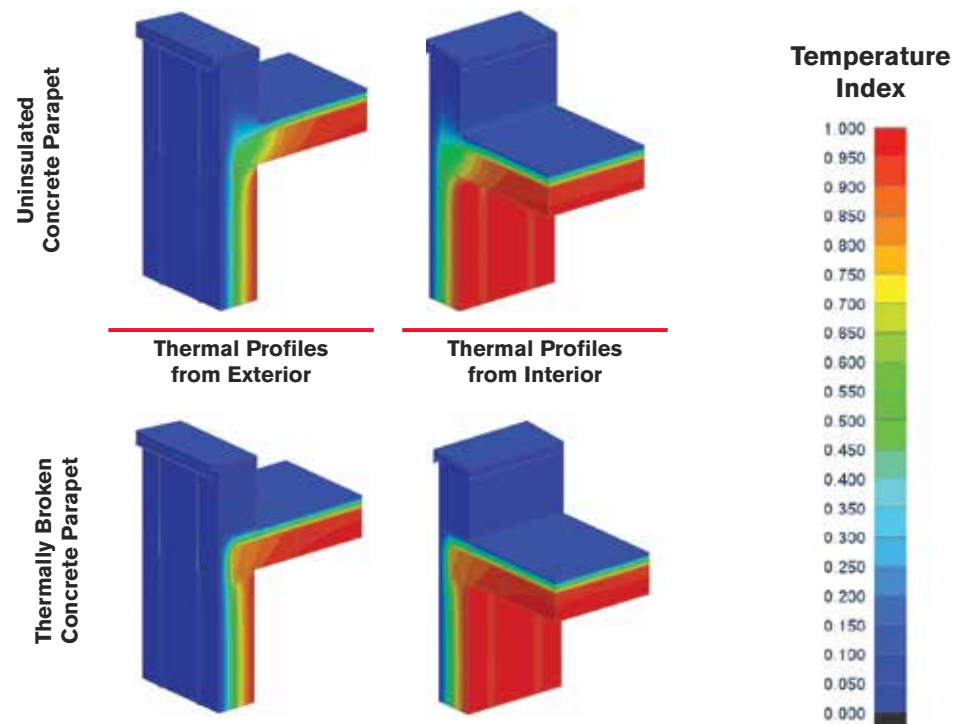
(5" Exterior Insulation and R-20 Batt Insulation scenario shown)
