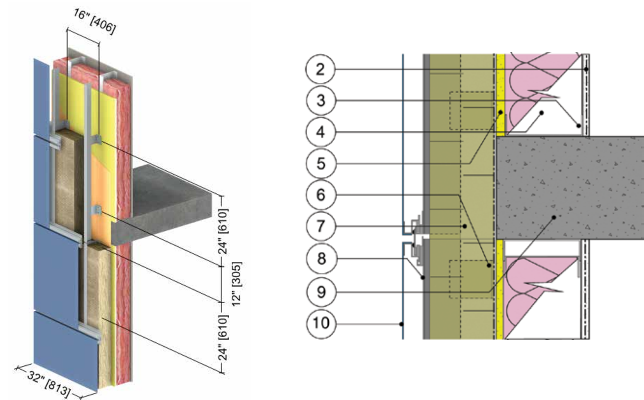
Exterior Insulated 2" x 6" Steel Stud (16" o.c.) Wall Assembly with Thermally Isolated Vertical Brackets and Rail System (24" o.c.) Supporting Metal Cladding – Intermediate Floor Intersection
