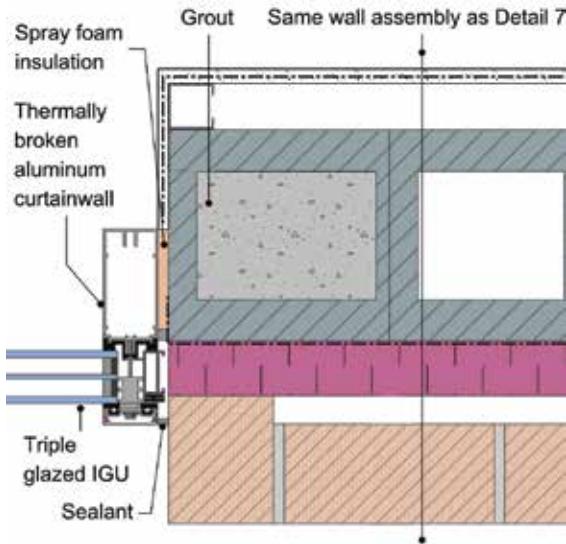
Jamb – Scenario B (2" Insulation)
