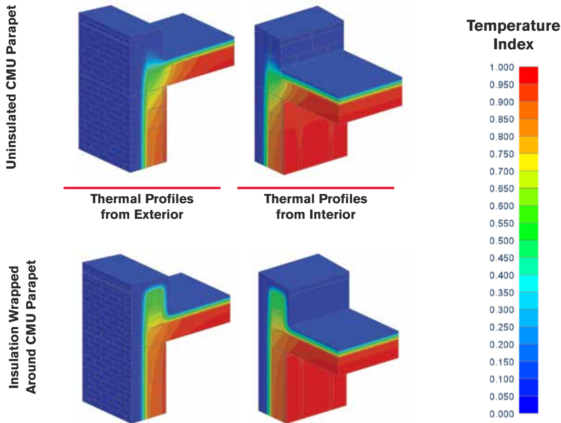
(4" Exterior Insulation scenario shown)
