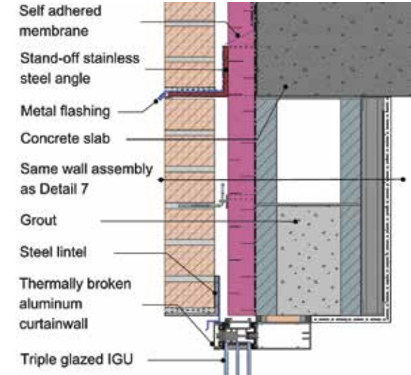
Head – Scenario B
