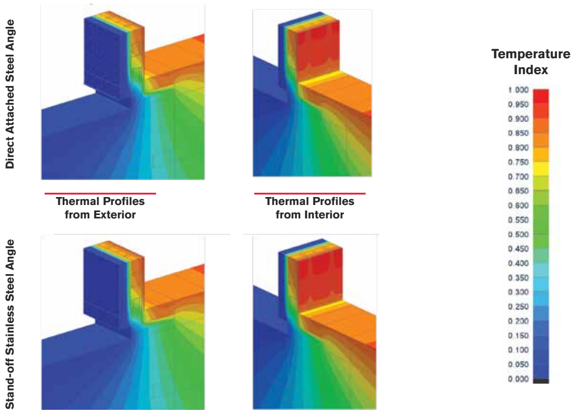
(4" Exterior Insulation scenario shown)
