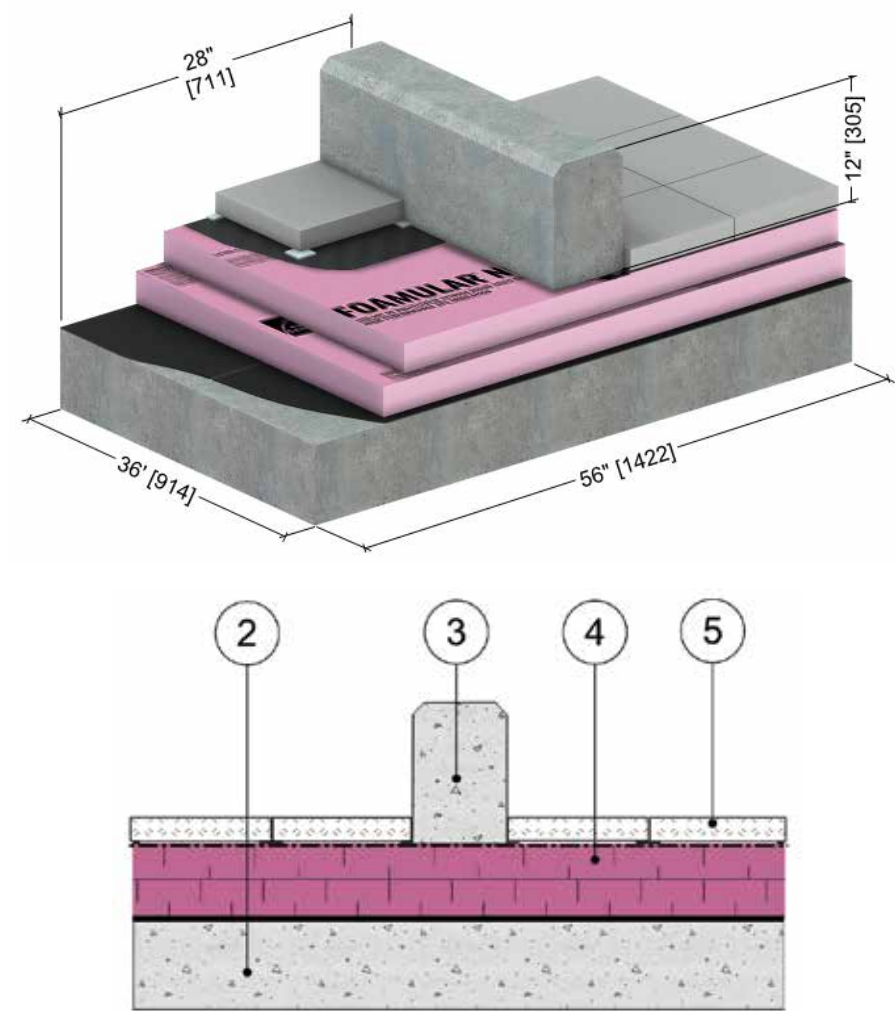
Insulated Protected Membrane Roof – Floating Concrete Wall Intersection
