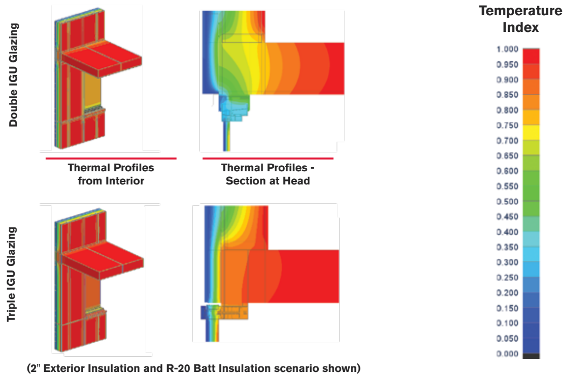
(2" Exterior Insulation and R-20 Batt Insulation scenario shown)
