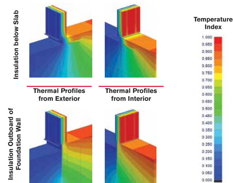
(5" Exterior Insulation and R-20 Batt Insulation scenario shown)
