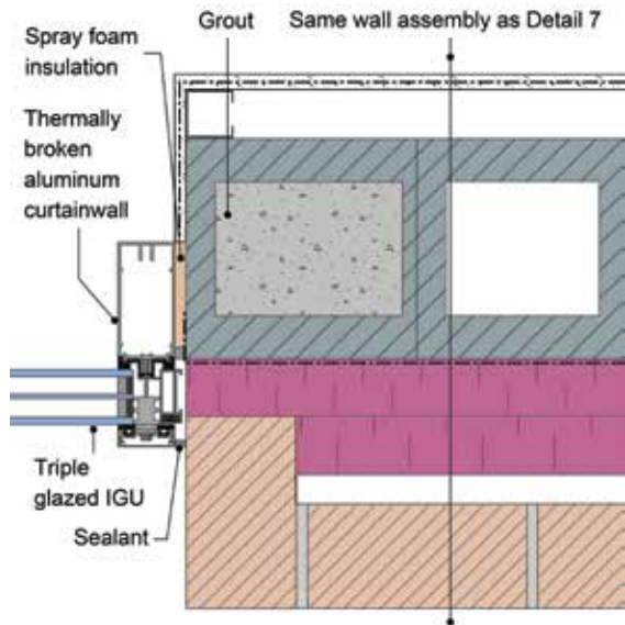
Jamb – Scenario B (4" Insulation)
