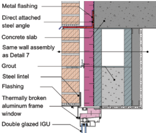
Head – Scenario B
