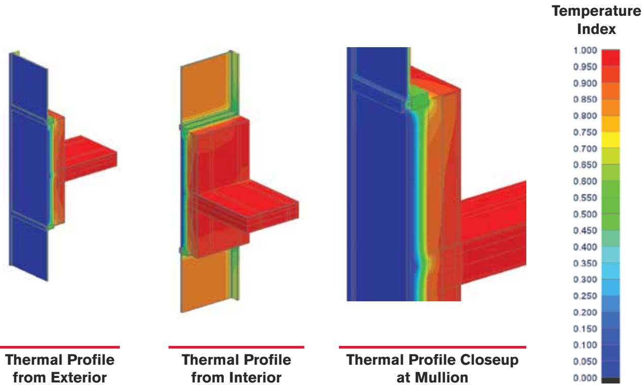
(4" spandrel insulation shown)
