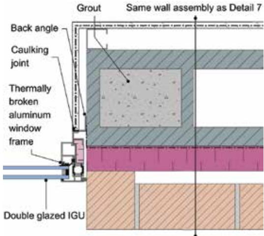
Jamb – Scenario A (2" Insulation)
