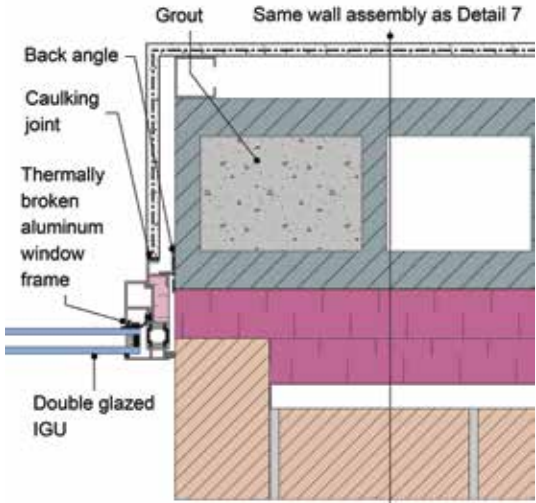
Jamb – Scenario A (4" Insulation)
