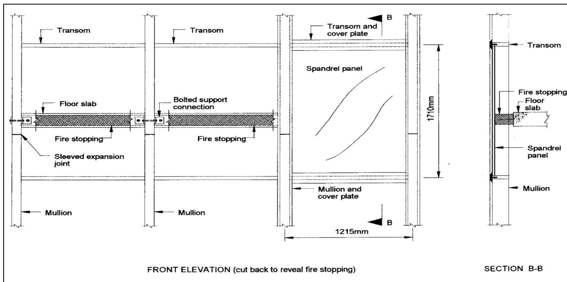
Fig.1 – Typical curtain wall system panel
