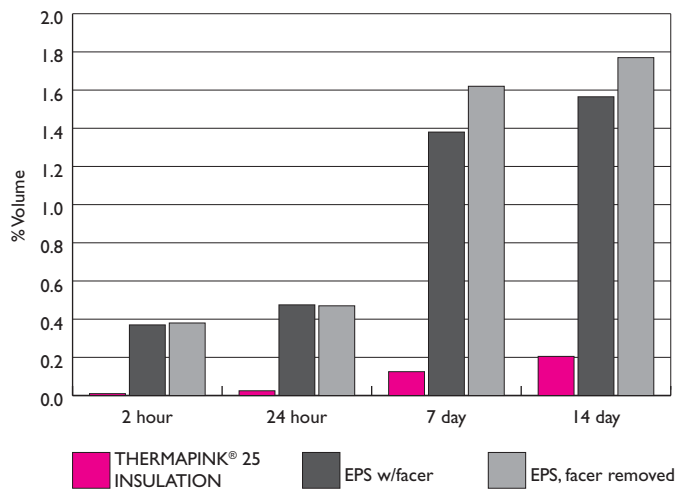
FIGURE 2—WATER ABSORPTION, XPS VS. EPS
