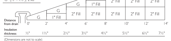
Typical Tapered Roofing Section, 1/2" per foot slope
