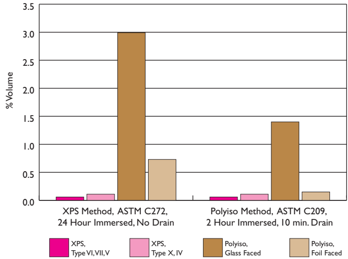
FIGURE 1—WATER ABSORPTION, XPS VS. POLYISO
