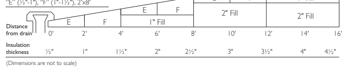
Typical Tapered Roofing Section, 1/4" per foot slope
